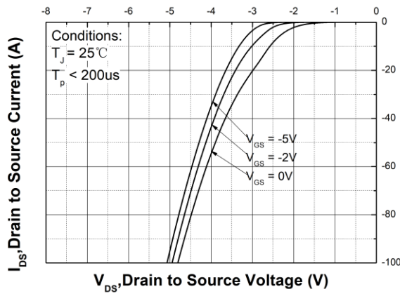
Figure 9. Body Diode Characteristic at T_J = 25^\circ C
