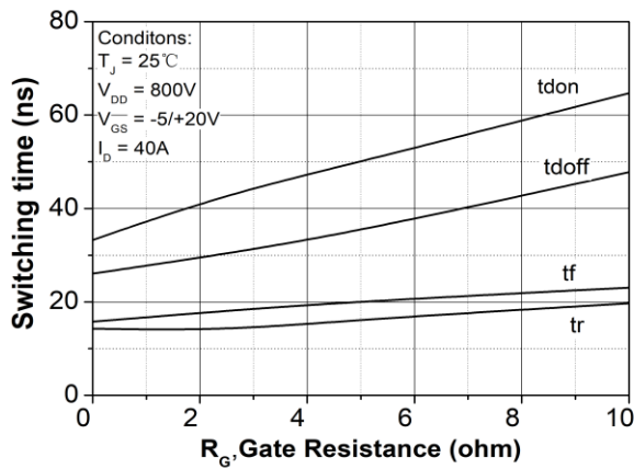
Figure 27. Switching Times vs. R_{G(\text{ext})}
